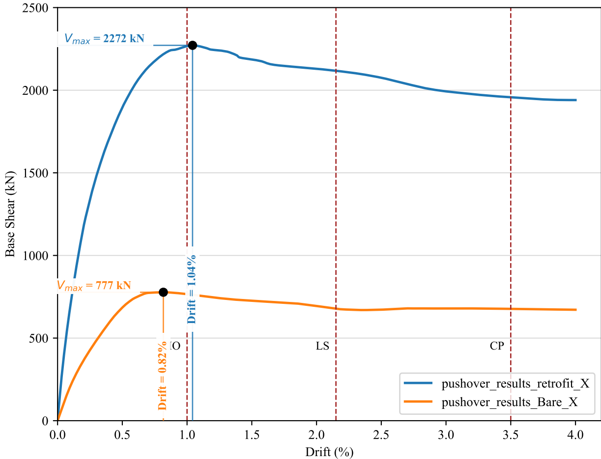
Pushover Curves
